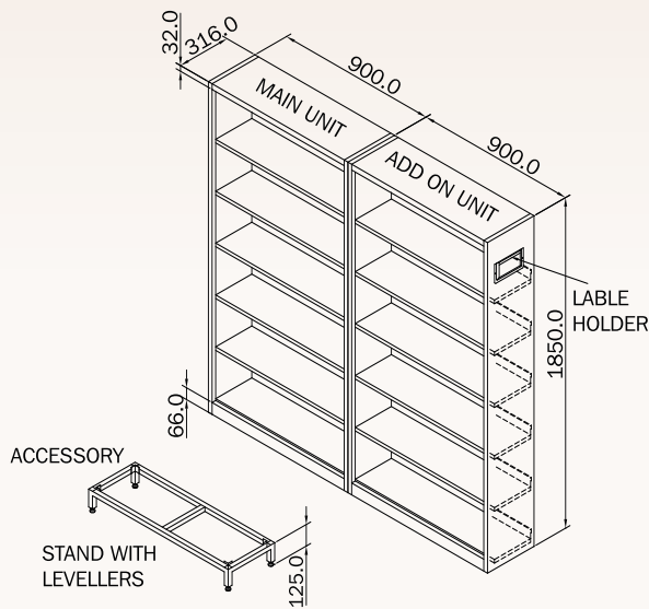
SINGLE SIDED STEEL BOOKRACK
