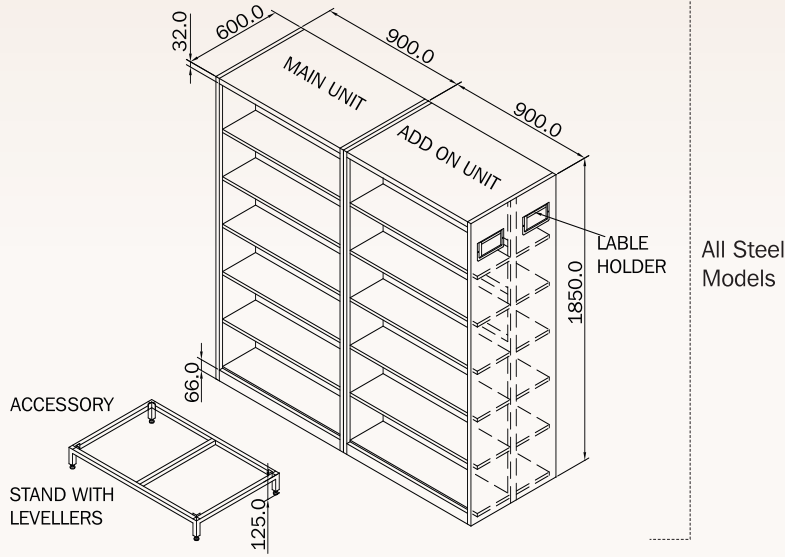
DOUBLE SIDED STEEL BOOKRACK
