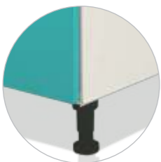
The cabinets are mounted on sturdy, height adjustable black plastic legs of diameter 40 mm, with a load bearing capacity of 450 KG/leg
