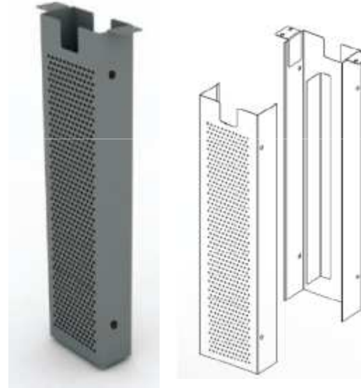
Vertical Wire Carrier
