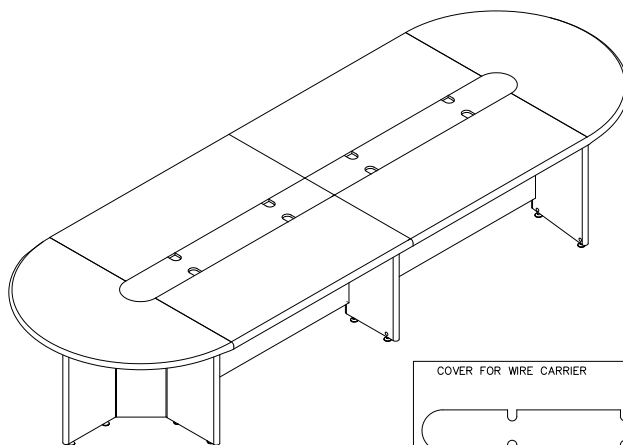
12-SEATER WITH WIRE CARRIER
